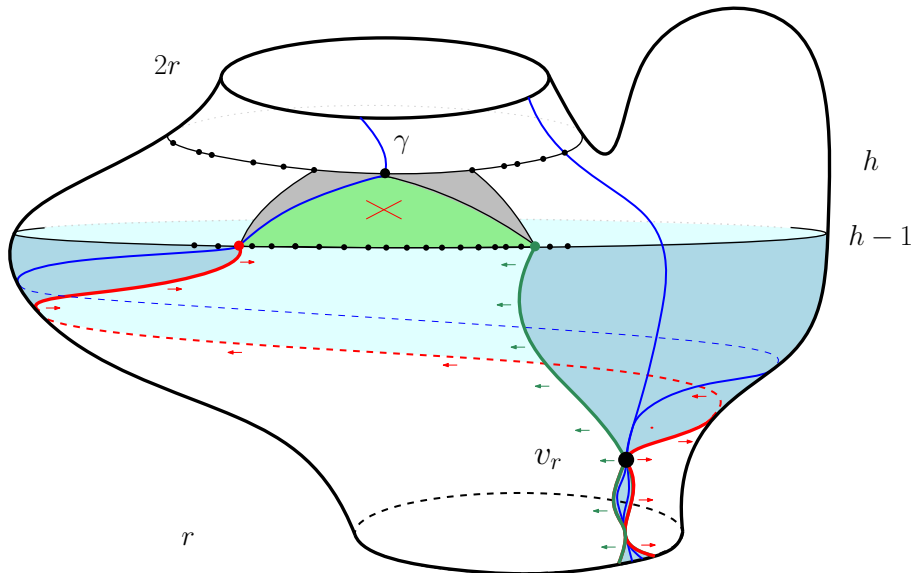
Figure 4.3. Illustration of the geometric event \mathcal{G}_r enforcing coalescence at scale r . We see the creation of a large slot (in green) whose perimeter is comparable to the total perimeter at level h \geq 3r/2 . We then enforce that the left-most geodesic (in red) and the right-most geodesic (in green) starting from the bottom corners of that slot meet before height r . Any geodesics towards the origin coming down from level 2r must live in the blue region and in particular must go through v_r .
