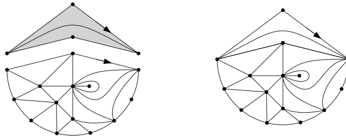
Figure 4.4. Illustration of the construction of a triangulation of the p -gon having no edge between the origin and non adjacent boundary vertices.
