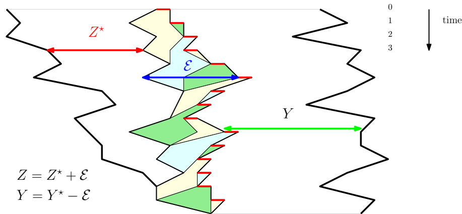
Figure 4.5. Illustration of the proof of Lemma 4.9 : at each generation step, one particle (in red) is stolen to Y to be reassigned to Z . The families of offspring of these migrants are depicted with different colors. Their aggregation forms the process \mathcal{E} which is negligible compared to Y and Z .
