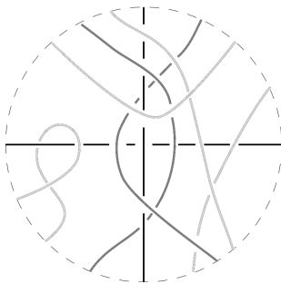
Figure 5.1. The link diagram of the curve from Example 5.2 together with two lines of hyperbolicity giving rise to different degree partitions.
