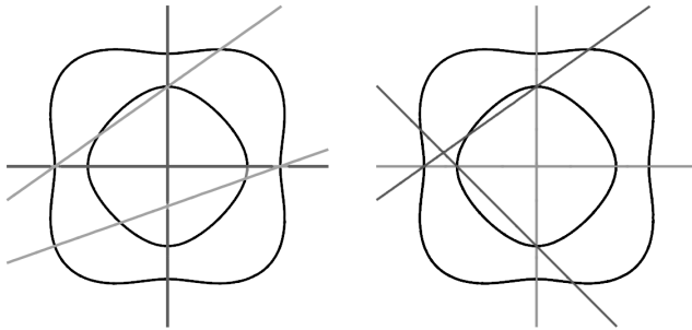
Figure 3.1. Realizing (3, 2) and (1, 3) with pencils of conics having 3 and 4 base points on X(\mathbb{R}) .
