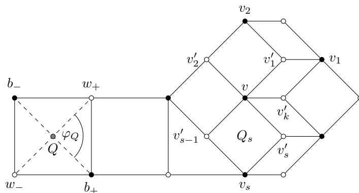
Figure 3.1: Bipartite quad-graph with notations
