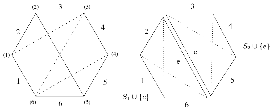
FIGURE 3. Decomposition of the hexagon on setting u_{25} = 0 . The variables corresponding to chords which cross \{2, 5\} , namely u_{13}, u_{46}, u_{14}, u_{36} , are all equal to 1 (left). The system (2.10) splits into the pair of equations, u_{15} = 1 - u_{26} and u_{35} = 1 - u_{24} , which identifies D_{25} with \mathfrak{M}_{0,4}^\delta \times \mathfrak{M}_{0,4}^\delta .
