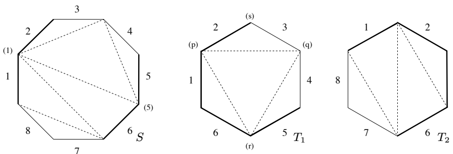
FIGURE 7. The induction step in the proof of Proposition 2.22. The chord \{1, 5\} in the octagon on the left distinguishes the four thick edges E = \{1, 2, 5, 6\} . The two sets T_1 = \{1, 2, 3, 4, 5, 6\} and T_2 = \{5, 6, 7, 8, 1, 2\} intersect in E and define the hexagons on the right. The right hand hexagon can be further decomposed into a pair of pentagons, but the middle hexagon has an internal triangle, so we have to invoke the triangle lemma 2.17. In this way, we reduce to the case of \mathfrak{M}_{0,6}^\delta and \mathfrak{M}_{0,5}^\delta only.
