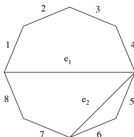
FIGURE 4. A partial decomposition \alpha \in \chi_{8,\delta}^2 of an octagon gives an isomorphism of D_\alpha with \mathfrak{M}_{0,5}^{\delta_1} \times \mathfrak{M}_{0,4}^{\delta_2} \times \mathfrak{M}_{0,3}^{\delta_3} = \mathfrak{M}_{0,5}^{\delta_1} \times \mathbb{A}^1 \times \{\text{pt}\} .
