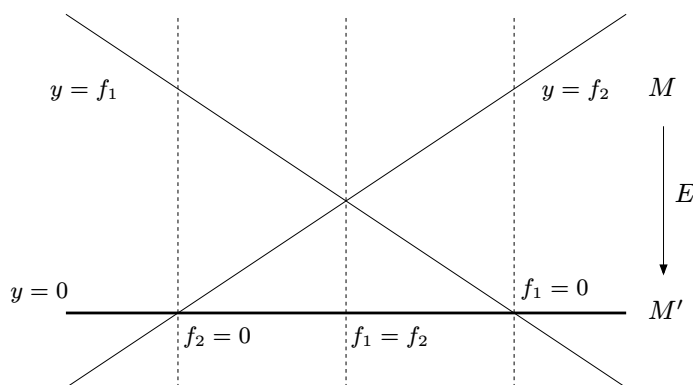
FIGURE 12. An arrangement M in \mathbb{A}^\ell which fibres over M' \subset \mathbb{A}^{\ell-1} (the thick line at the bottom). A vertical hyperplane (dashed) passes through every point where horizontal hyperplanes intersect.
