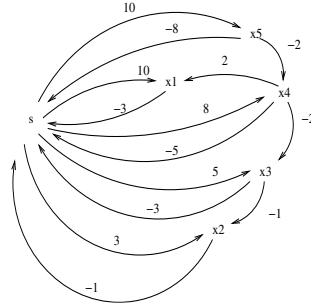
FIGURE 1. Distance graph associated to the CSP
