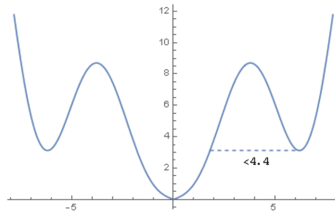
FIGURE 1. Illustration of the global convergence condition
