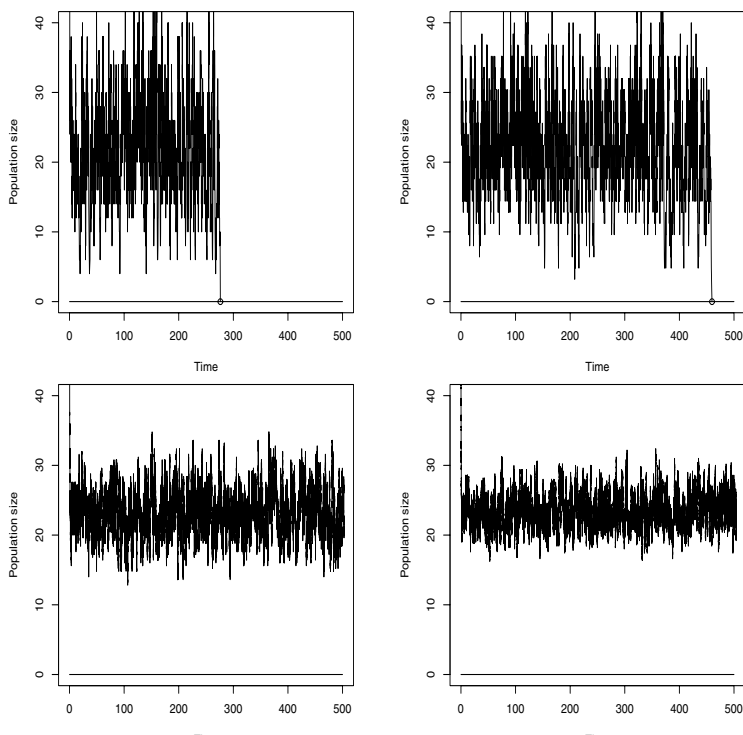
FIGURE 3. Simulation of a logistic age-structured population under different renormalizations ( n = 1, n = 1.25, n = 5, n = 10 ).
