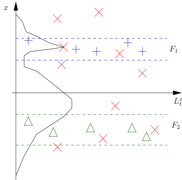
FIGURE 2. (Color online) Representation of the Poisson random measure \Delta in terms of \Delta_\wedge, \Delta_1 and \Delta_2 , represented by \times, + and \triangle respectively.
