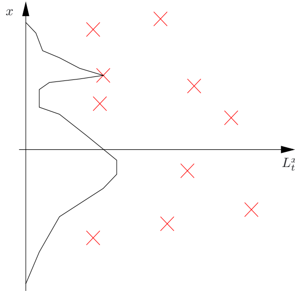
FIGURE 1. (Color online) The curve on the left represents the local time L_t^x at time t . As time increases, the curve moves outwards. The crosses are distributed according to \Delta and T occurs the first time the local time curve hits such a point.
