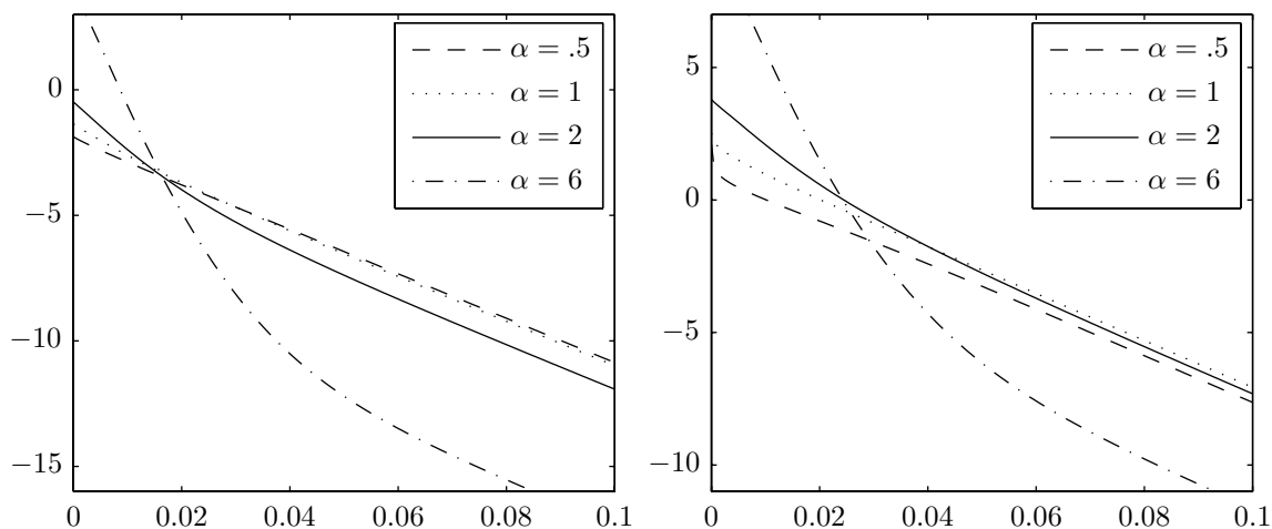
FIGURE 7. The natural logarithm of the entropies \log(E_\alpha^d[u](t)) (left) and \log(F_\alpha^d[u](t)) (right) versus time for different values of \alpha ( \beta = 1/2 , d = 2 ).
