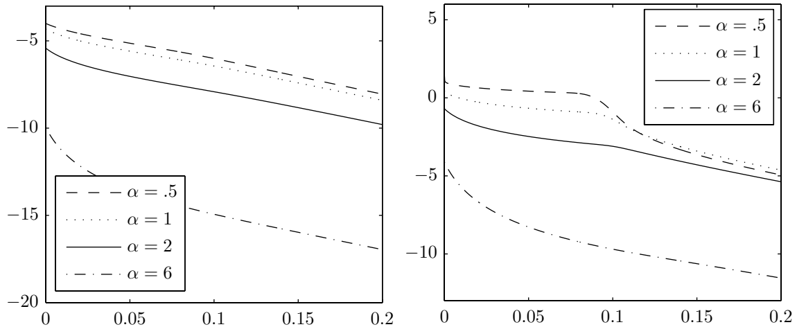
FIGURE 3. The natural logarithm of the entropies \log(E_\alpha^d[u](t)) (left) and \log(F_\alpha^d[u](t)) (right) versus time for different values of \alpha ( \beta = 2 , d = 1 ).
