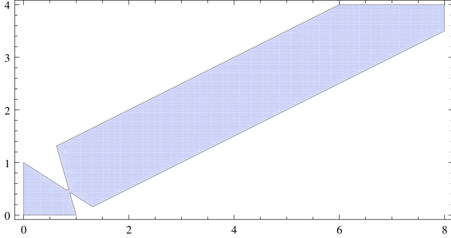
FIGURE 1. Illustration of the set M_d , defined in Theorem 5.2, for d = 9 .
