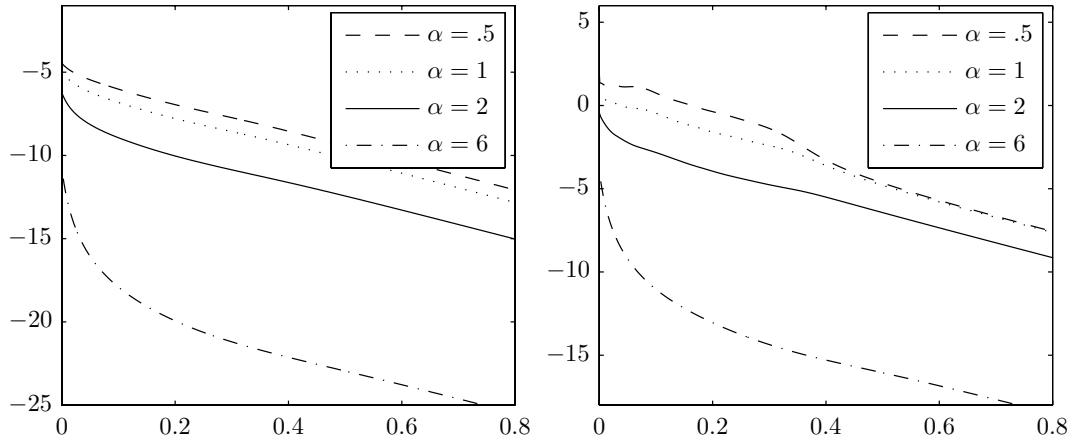
FIGURE 5. The natural logarithm of the entropies \log(E_\alpha^d[u](t)) (left) and \log(F_\alpha^d[u](t)) (right) versus time for different values of \alpha ( \beta = 2, d = 2 ).
