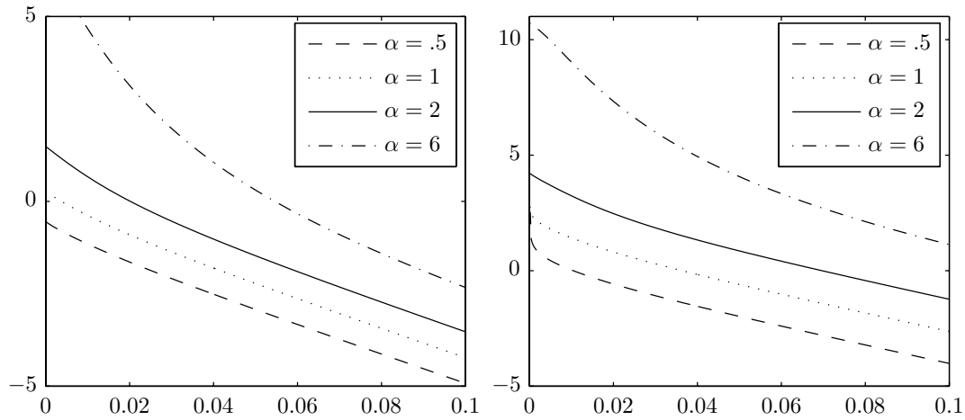
FIGURE 6. The natural logarithm of the entropies \log(E_\alpha^d[u](t)) (left) and \log(F_\alpha^d[u](t)) (right) versus time for different values of \alpha ( \beta = 1/2, d = 1 ).
