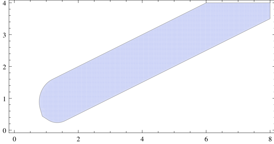
FIGURE 2. Set of all (\alpha, \beta) fulfilling s_0 \geq 0 , (5.5), and (5.6) for d = 9 .
