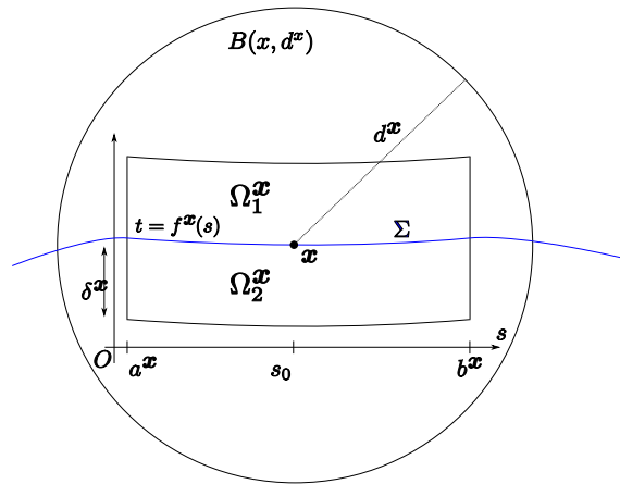
FIGURE 6. Situation in a neighborhood of x .
