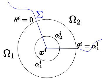
FIGURE 4. Notations for x^i \in \mathcal{S}_{\text{int}} - \alpha^i = \alpha_2^i .
