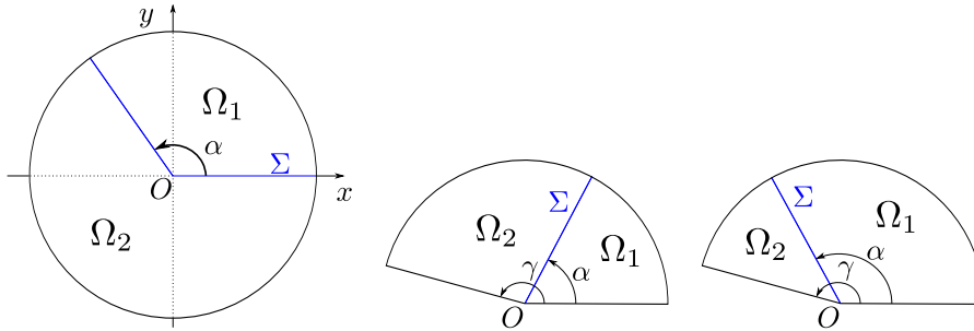
FIGURE 2. (left) Geometry of an interior vertex. (middle, right) Geometries of a boundary vertex.
