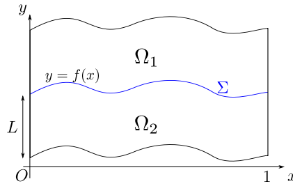
FIGURE 3. Geometry for an interface of \mathcal{C}^1 -class.
