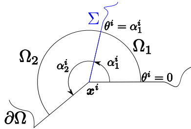
FIGURE 5. Notations for x^i \in \mathcal{S}_{\text{ext}} - \alpha^i = \alpha_1^i .
