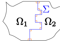
FIGURE 8. A is Fredholm of index 0 when \sigma_2/\sigma_1 \in \mathbb{R}^* \setminus [-3; -1/3] .
