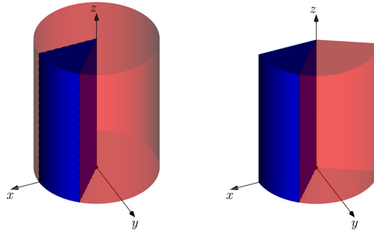
FIGURE 12. Geometry of prismatic edges: (left) interior edge. (right) Boundary edge.
