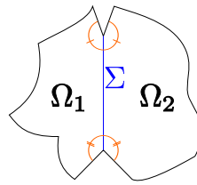
FIGURE 7. A is Fredholm of index 0 when \sigma_2/\sigma_1 \in \mathbb{R}^* \setminus \{-1\} .
