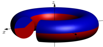
FIGURE 13. Geometry of an interior axisymmetric edge.
