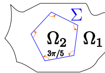
FIGURE 10. A is Fredholm of index 0 when \sigma_2/\sigma_1 \in \mathbb{R}^* \setminus [-7/3; -3/7] .
