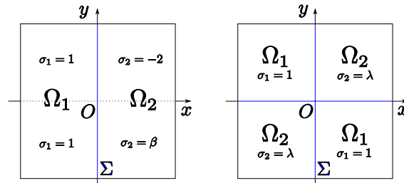
FIGURE 11. Two situations not covered by Theorem 4.3: \beta > -1 on the left; \lambda \in \mathbb{R}_-^* on the right.
