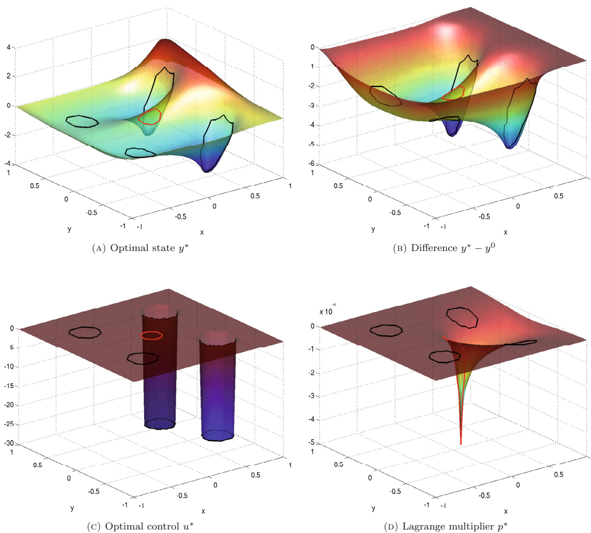
FIGURE 2. Results for unilateral constraint ( y|_{\omega_0} \leq c ).
