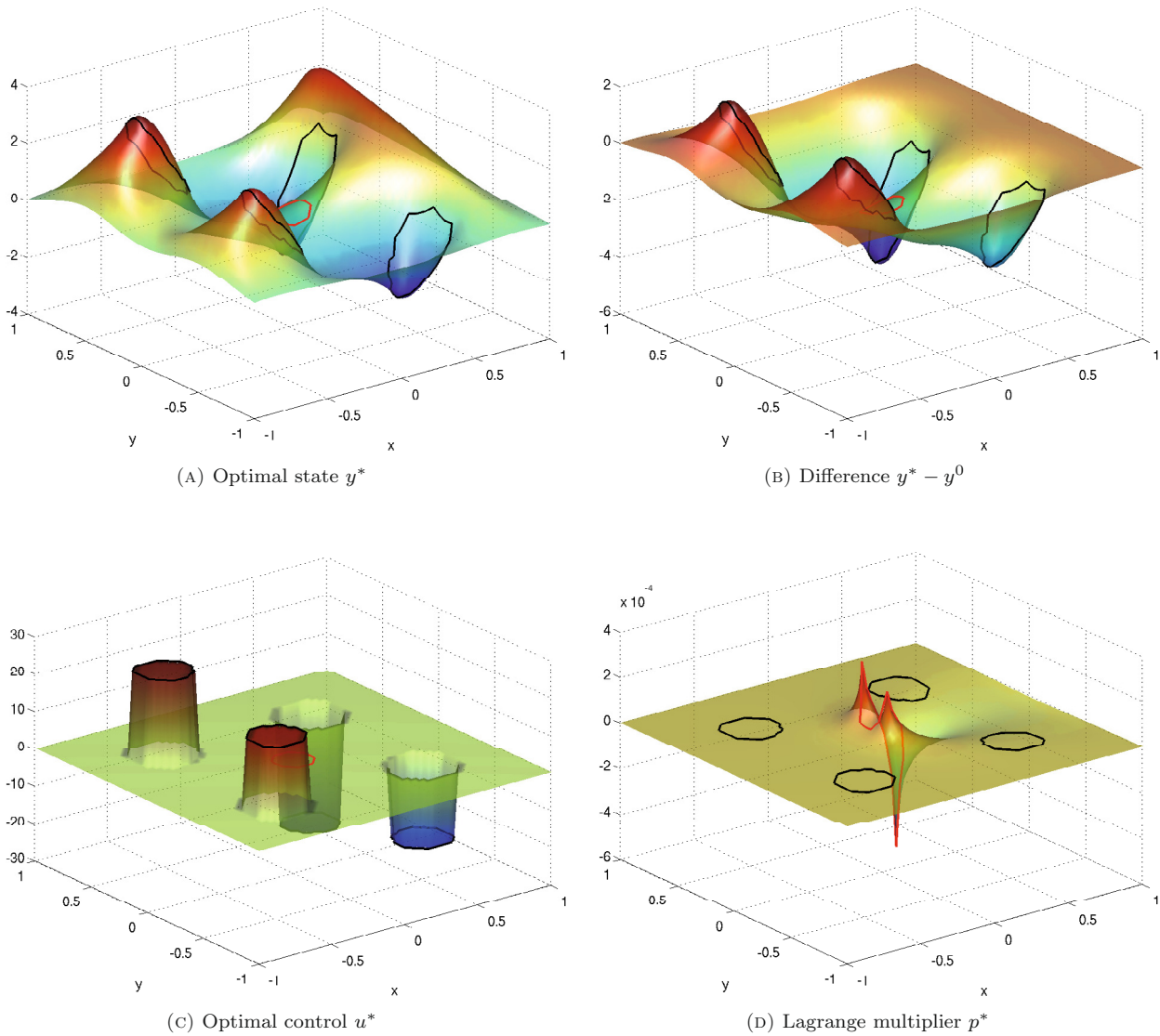
FIGURE 4. Results for L^\infty norm minimization ( \beta_1 = \beta_2 = 1 ).
