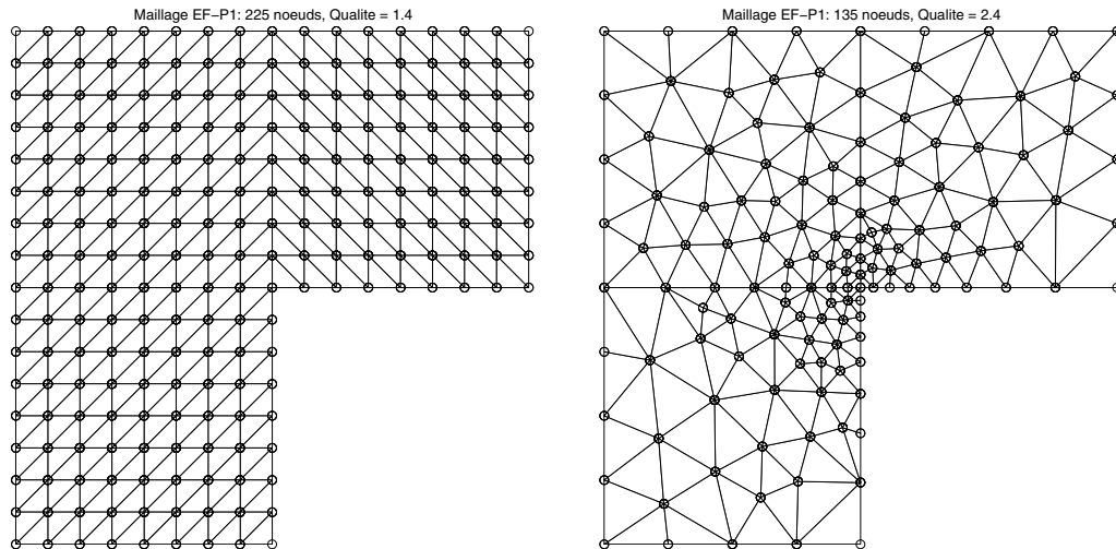
FIGURE 5. Example of meshes used for calculations. Left: uniform, 384 triangles (225 vertices in P_1 ). Right: geometric refinement, 228 triangles (135 vertices in P_1 ).
