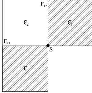
FIGURE 3. L-shaped domain with three subdomains.
