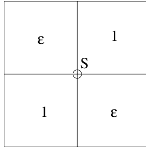
FIGURE 7. Checkerboard with four subdomains.
