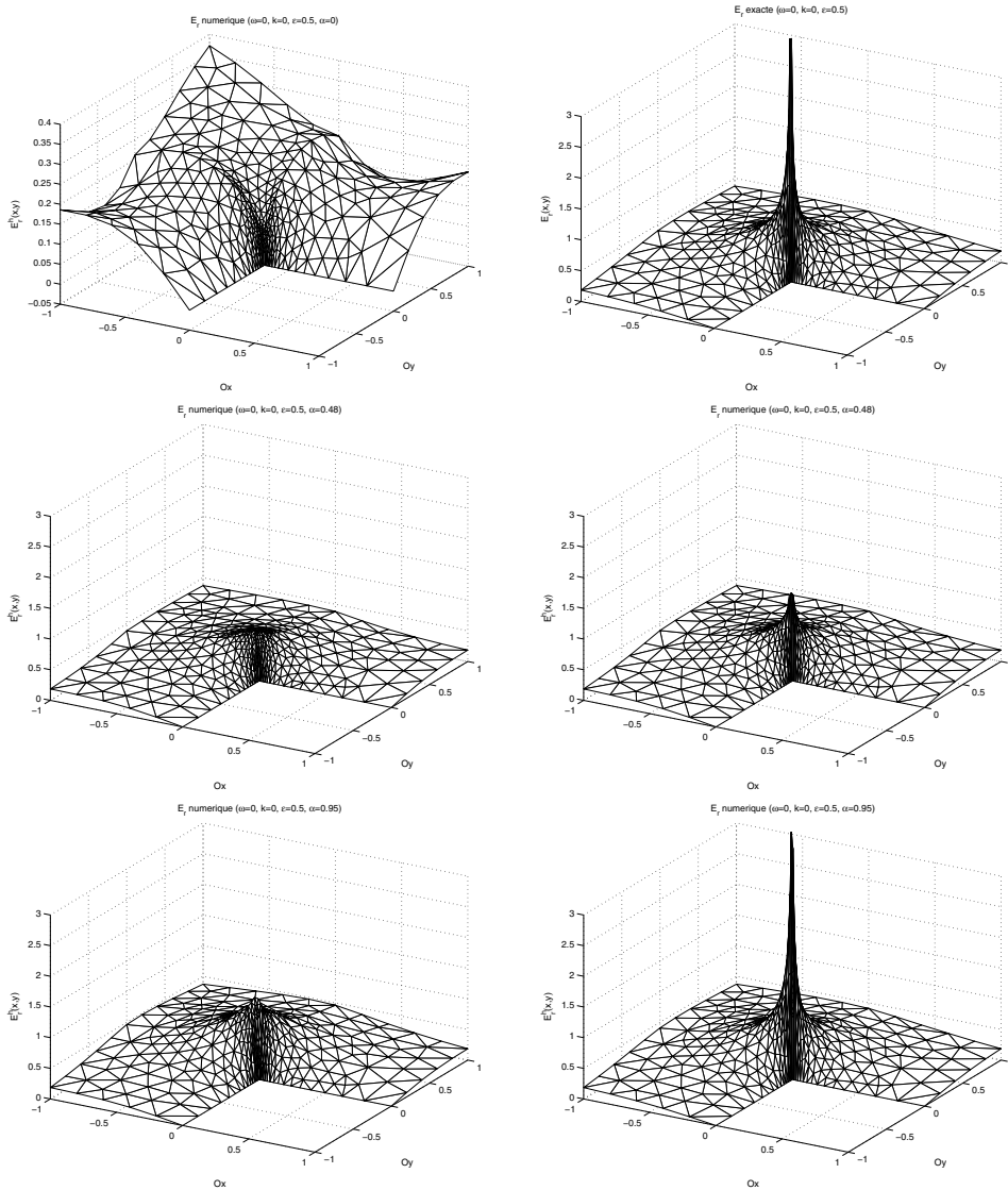
FIGURE 6. Radial component E_r of the singular solution: \varepsilon_1 = 0.5 , \varepsilon_2 = 1 , \varepsilon_3 = 0.5 with the same refined mesh of 564 triangles (314 vertices in P_1 , 1191 vertices in P_2 ). Top left: P_1 solution with standard regularization ( \alpha = 0 ). Top right: exact solution. Middle: P_1 (left) and P_2 (right) solution with weighted regularization ( \alpha = 0.48 ). Bottom: P_1 (left) and P_2 (right) solution with weighted regularization ( \alpha = 0.95 ).
