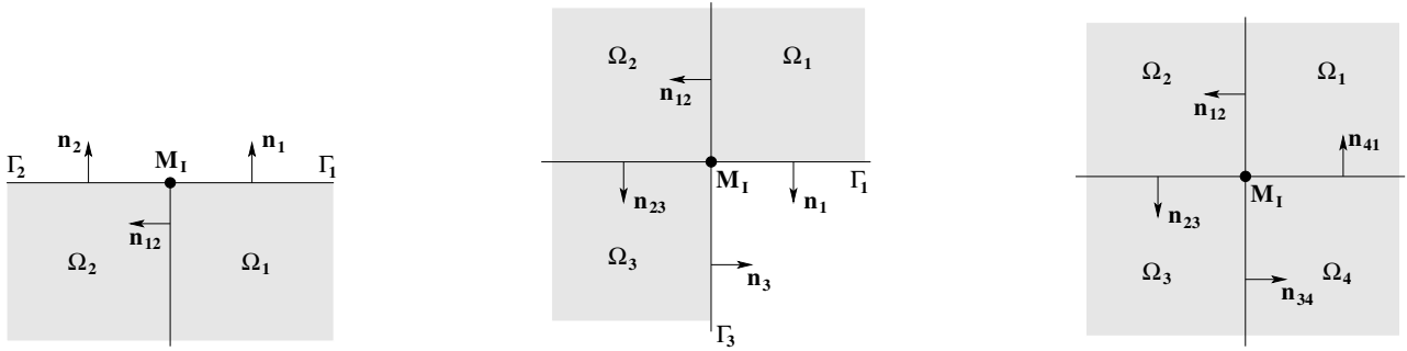
FIGURE 2. Boundary and transmission conditions at vertices.
