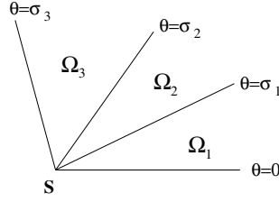
FIGURE 1. Subdomains having a common vertex ( J_S = 3 ).
