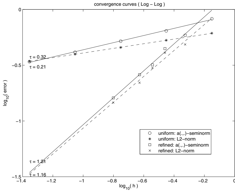
FIGURE 4. Singular solution: numerical rates of convergence for the P_1 -FEM with uniform and refined meshes.
