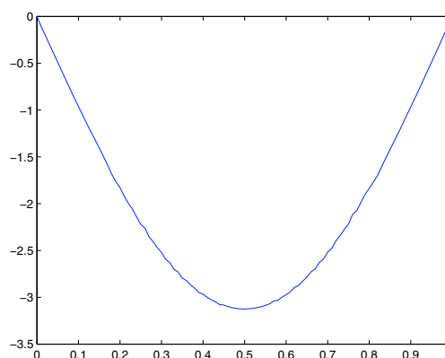
FIGURE 7. \bar{u}_{\tau h} at c = 0.5 .
