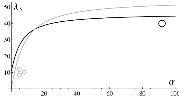
FIGURE 3. Robin optimisers for \lambda_3 .
