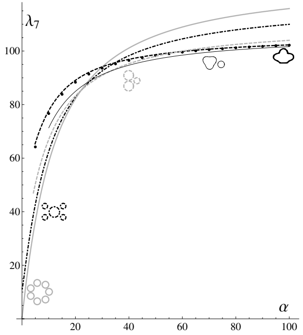
FIGURE 7. Robin optimisers for \lambda_7 .
