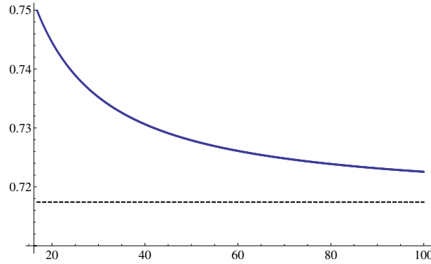
FIGURE 4. Area of the largest ball of \Omega_4^* .
