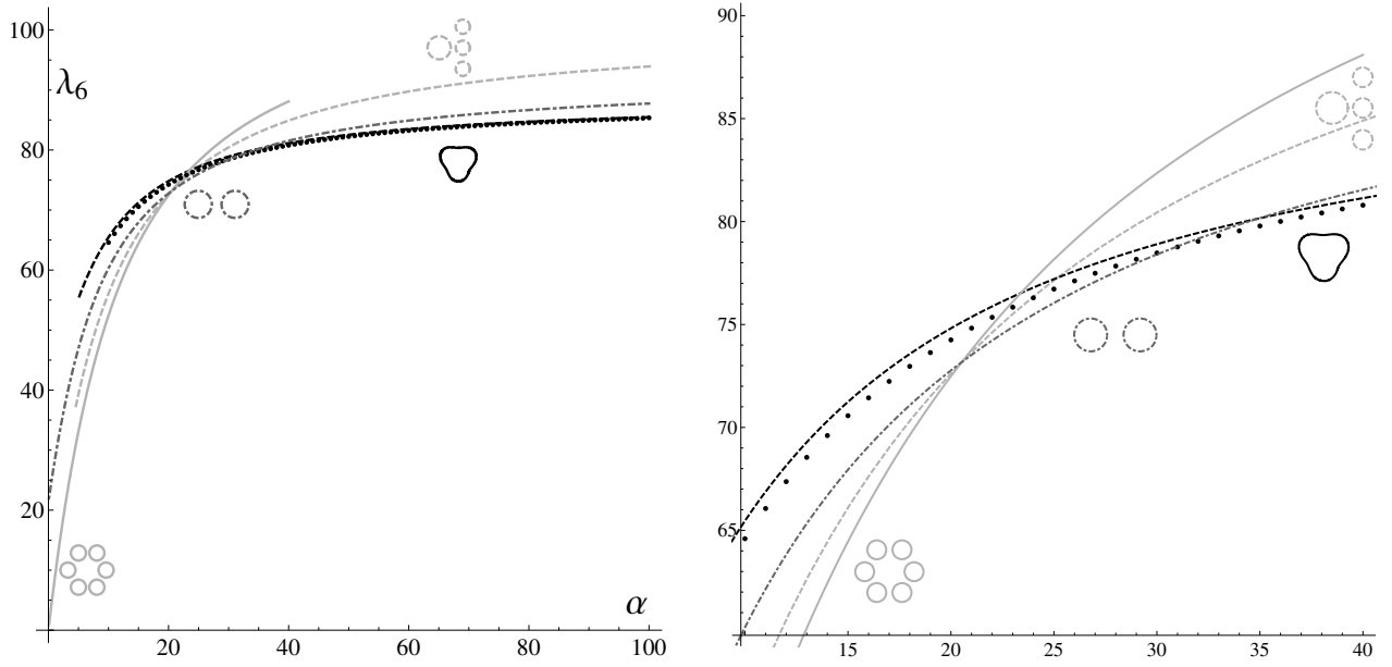
FIGURE 6. Robin optimisers for \lambda_6 and a zoom of the region associated with \alpha \in [10, 40] .
