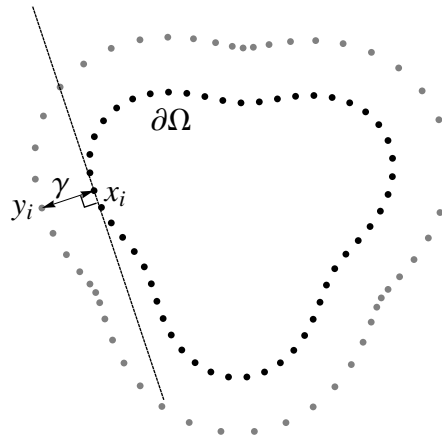
FIGURE 1. The collocation and source points.
