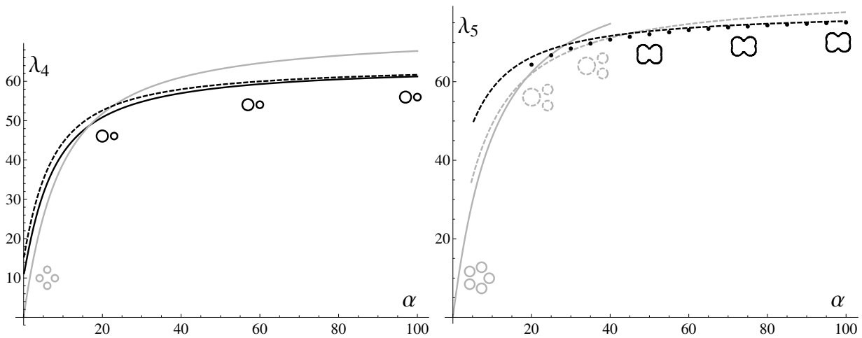
FIGURE 5. Robin optimisers of \lambda_4 and \lambda_5 .
