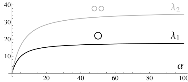
FIGURE 2. Robin optimisers for \lambda_1 and \lambda_2 .
