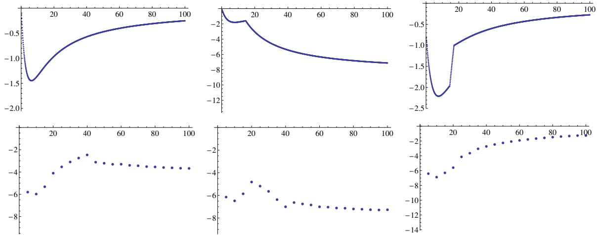
FIGURE 8. Numerical values for bound (2.13) with n=1,2,\dots,6 .
