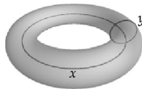
Fig. 2. Cell structure of the 2-torus.
