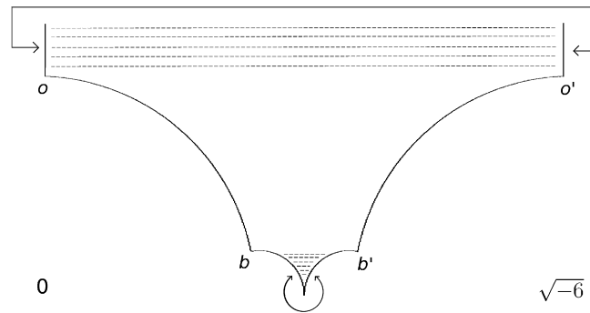
Fig. 1. Intersection of the fundamental polyhedron for SL_2(\mathcal{O}_{\mathbb{Q}(\sqrt{-6})}) with the imaginary upper half-plane. The intersections with the translates of \mathcal{F} are indicated by the dashed lines.
