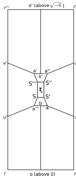
Fig. 3. Bottom facets for SL_2(\mathcal{O}_{\mathbb{Q}(\sqrt{-6})}) .
