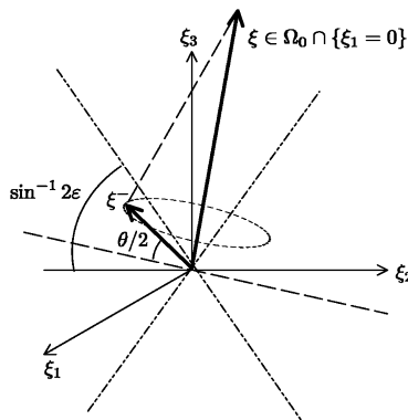
Fig. 4. \xi \in \Omega_0 and \xi^- almost orthogonal to \xi_3 .
