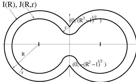
Fig. 2. Definitions of I(R) and J(R, r) .
