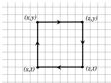
FIG. 2. — The curve \hat{q}
