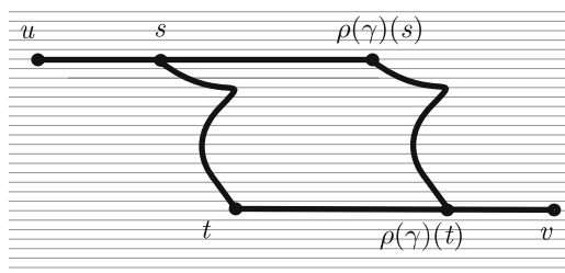
FIG. 3. — The \pi -curves C and \tilde{c}
