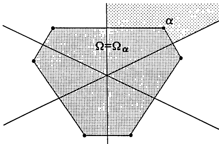
Fig.4 shows a weight diagram of any positive weight \alpha in the Weyl chamber (lightly shaded sector) of Lie algebra \mathfrak{G} = \mathfrak{su}(3) . The same figure describes restricted weights of symmetric space SU(3)/SO(3) . The G -orbit of element \alpha in \mathfrak{su}(3) projects down onto its weight-diagram (the dark shaded region \Omega = \Omega_\alpha ), the convex hull of \alpha , reflected by all elements of the Weyl group W of \mathfrak{su}(3) .
