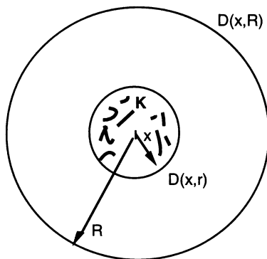
Figure 2 : Elimination Lemma
