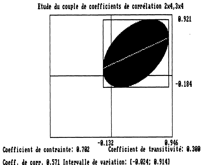
FIGURE 2 Ensemble de variation du couple (r_{2,4}, r_{3,4})
