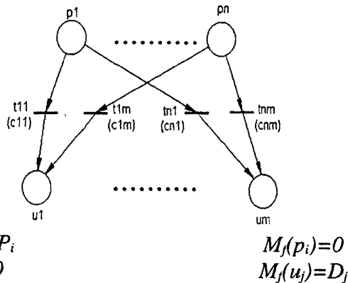
Figure 2. – The generic Petri net model of the STP (the mutual exclusion place is not drawn).
