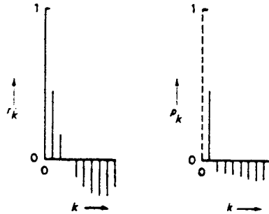
Figure 11. — Complete correlation patterns for the Box and Jenkins simulation.
