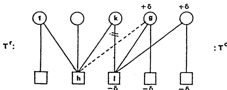
Figure 2. — A spanning tree T and subtrees T' , T^c ; values of new dual variables; (g, h) adjoined edge, (k, l) deleted edge.
