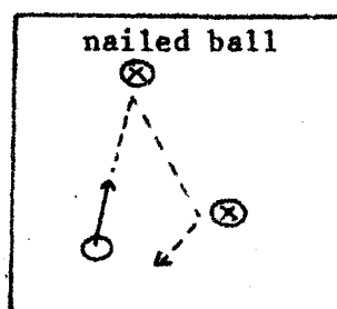
Sinai billiard
