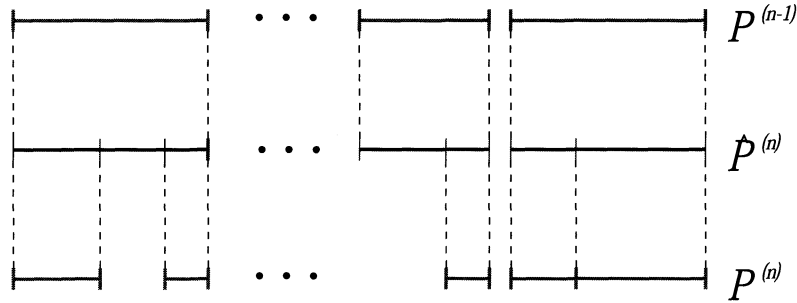
FIG. 3. — Creating \Omega^{(n)} from \Omega^{(n-1)}
