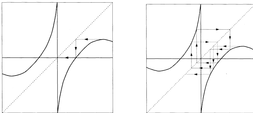
FIG. 2. — (a) At the bifurcation we have f_{c+\varepsilon}^2(\pm c) = 0 . (b) f_{c+\varepsilon+\eta}^2(\pm c) \neq 0
