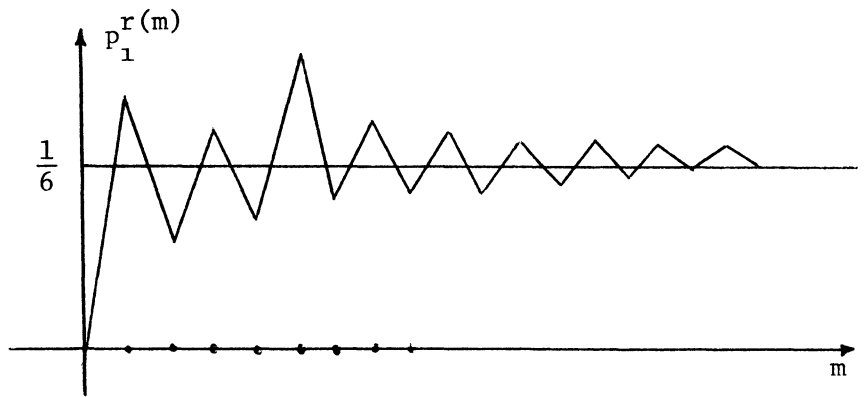
Fig. 7. Prior and observed probability
