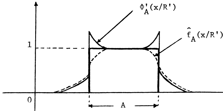
Fig. 4. Membership functions derived from relativistic characteristic function.
