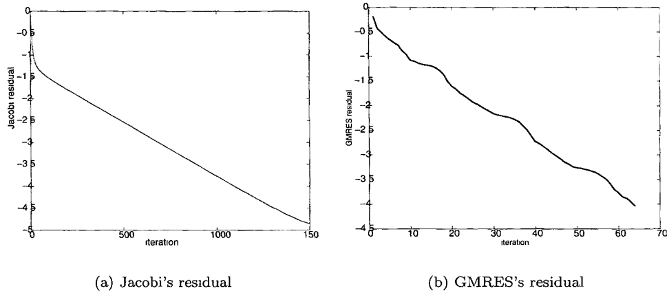
FIGURE 8. Residual for two different algorithms.
