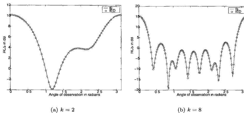
FIGURE 4. Bistatic RCS for the square geometry
