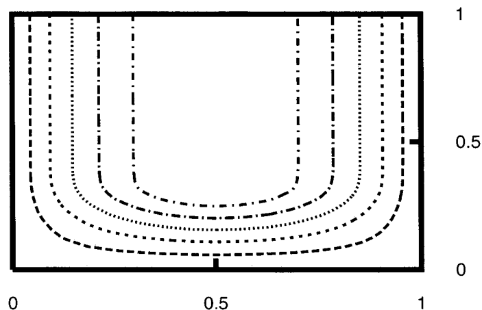
FIGURE 10. Contour lines of the approximation to the solution of the problem with \sigma(x, y) = 16[(x - 1/2)^2 + (y - 1/2)^2 - 1/16] and f(x, y) = 1 in Example 4. The solution is negative again with the inner contour being the minimum.
