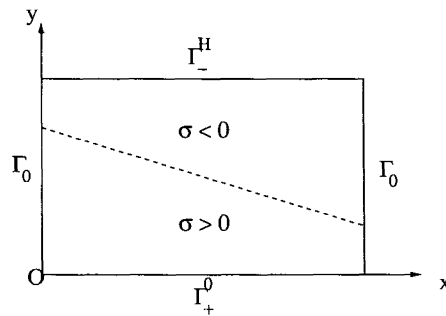
FIGURE 4. \sigma(x, y) = 3 - x - 5y .
