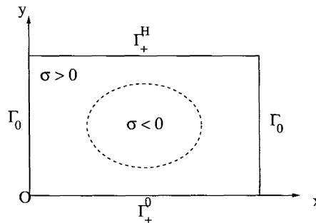
FIGURE 5. \sigma(x, y) = (x - 1/2)^2 + (y - 1/2)^2 - 1/16 .
