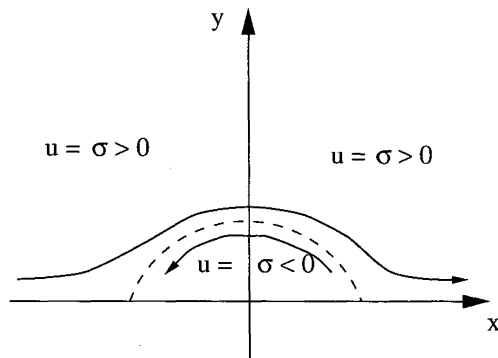
FIGURE 7. \sigma(x, y) = u , the first component of the velocity
