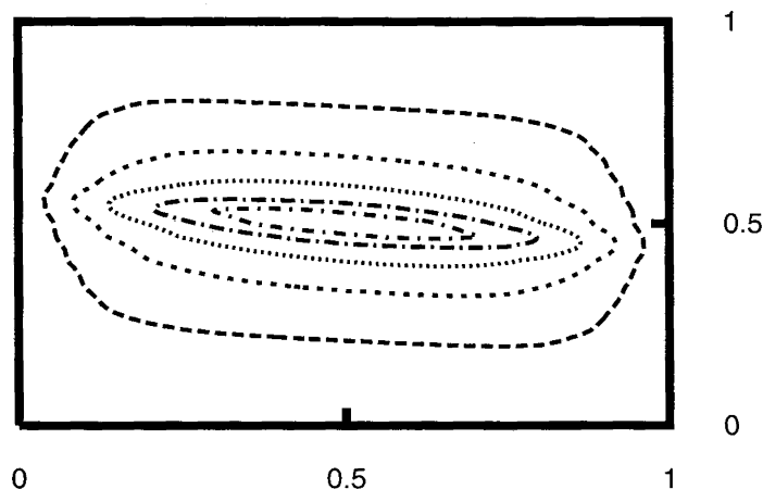
FIGURE 8. Contour lines of the approximation to the solution of the problem with \sigma(x, y) = 10(3 - x - 5y) and f(x, y) = 10 in Example 2. The solution is negative in this case and the value of the function decreases from the outer to inner contours.
