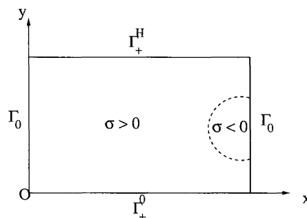
FIGURE 2. \sigma(x, y) = (x - 1)^2 + (y - 1/2)^2 - 1/16 .
