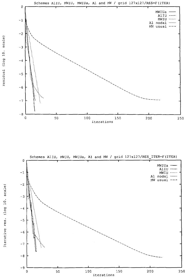
Figure 6. — Comparison of the methods MWIU, MWIUa, A1IU, A1 nodal and MW. The evolution of the residue and the iterative residue are plotted against the iterations. The grid is C_{1.6} ; \gamma = \nu = 120 , \varepsilon = 2 .
