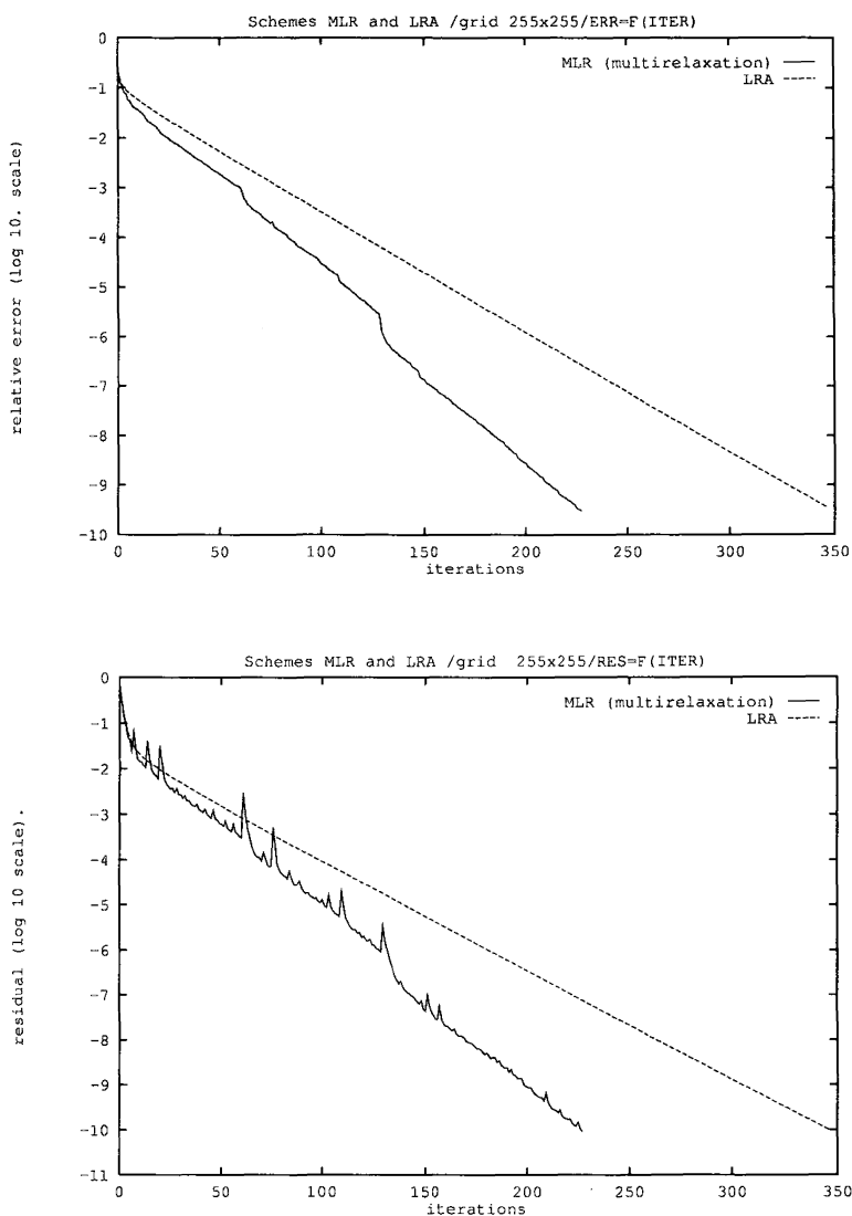
Figure 5. — Comparison between the LRA and MLR Methods. The relative error and the residue are plotted against iterations. The grid is C_{1.7} .
