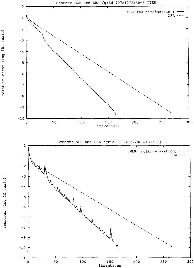
Figure 4. — Comparison between the LRA and MLR Methods. The relative error and the residue are plotted against iterations. The grid is C_{16} .
