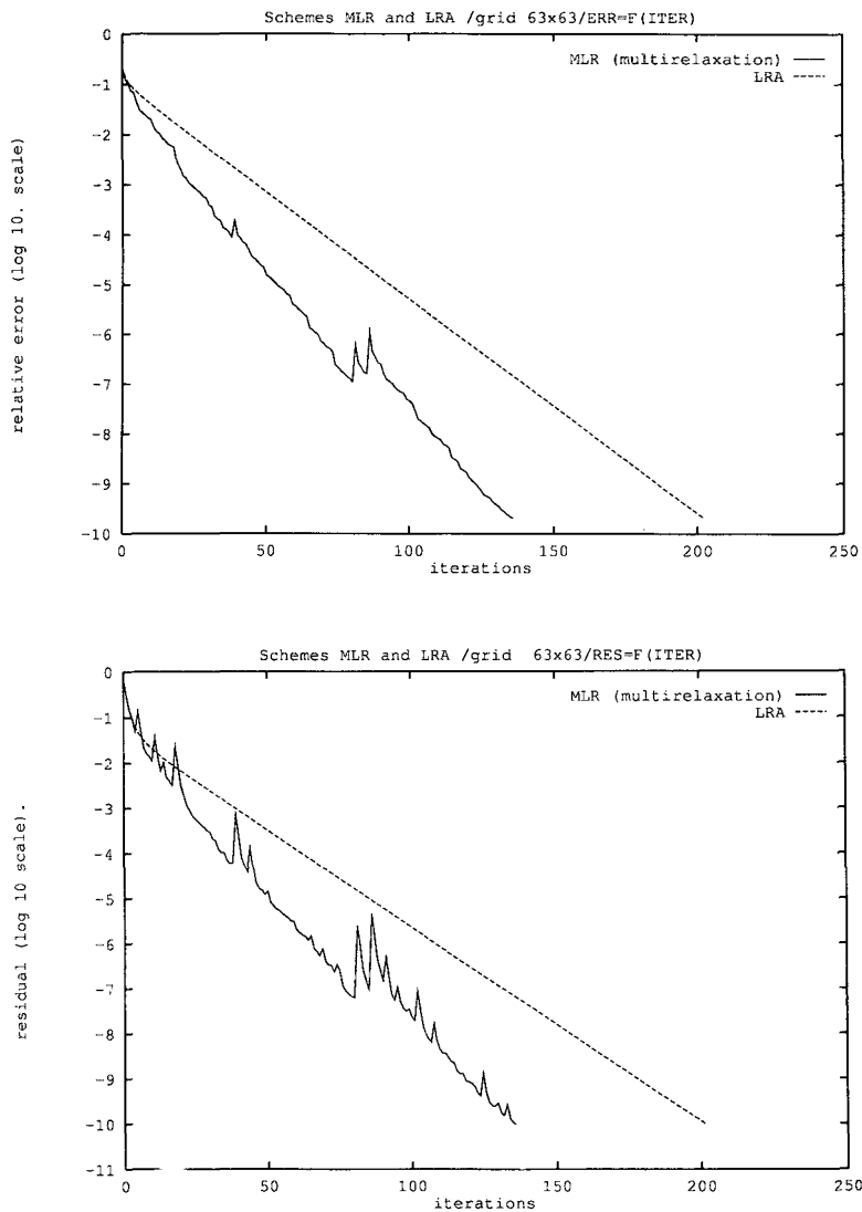
Figure 3. — Comparison between the LRA and MLR Methods. The relative error and the residue are plotted against iterations. The grid is C_{1.5} .
