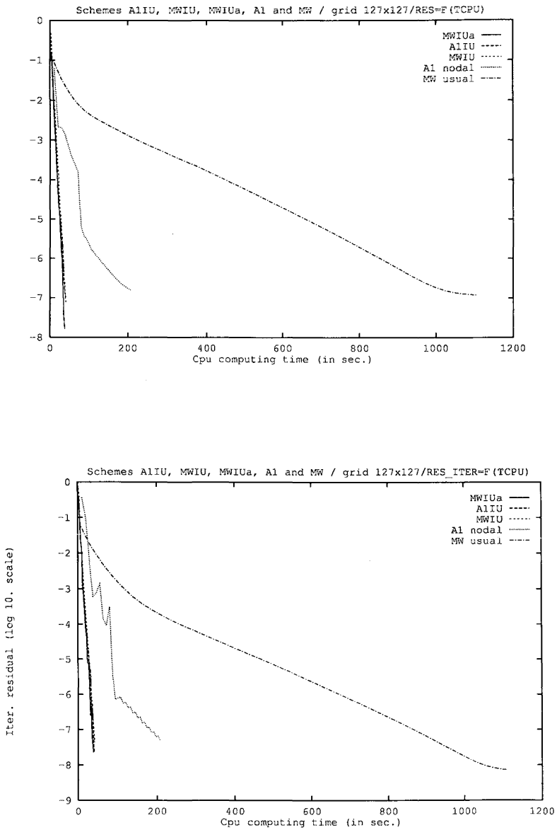
Figure 7. — Comparison of the methods MWIU, MWIUa, A1IU, A1 nodal and MW. The evolution of the residue and the iterative residue are plotted against the CPU time (in seconds). The grid is C_{16} ; \gamma = \nu = 120 , \varepsilon = 2 .
