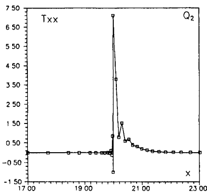
Figure 5. — Curves \sigma_{xx} \times x for the stick-slip problem along line y = D near point (L_1, D) of
