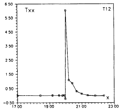
Figure 5. — Curves \sigma_{xx} \times x for the stick-slip problem along line y = D near point (L_1, D) of
