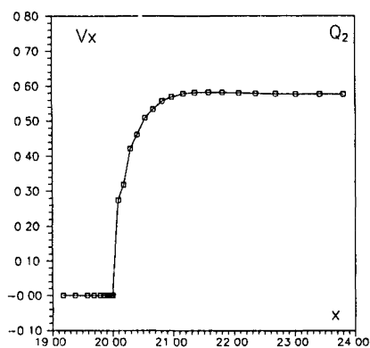
Figure 4. — Curves u_x \times x for the stick-slip problem along line y = D near point (L_1, D) of
