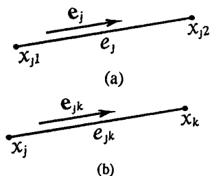
Figure 2.2. — Alternative notation for edges and their end-points.
