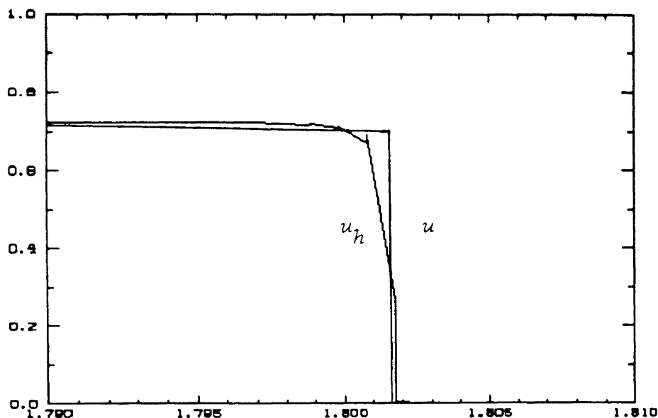
Figure 3.2b. — Detail of the convergence of the approximate solution determined by the \Lambda\Pi P^0 P^1 -scheme with \theta_i \equiv 1 , and cfl = 1/8 to the entropy solution of the Buckley-Leverett problem 3.
