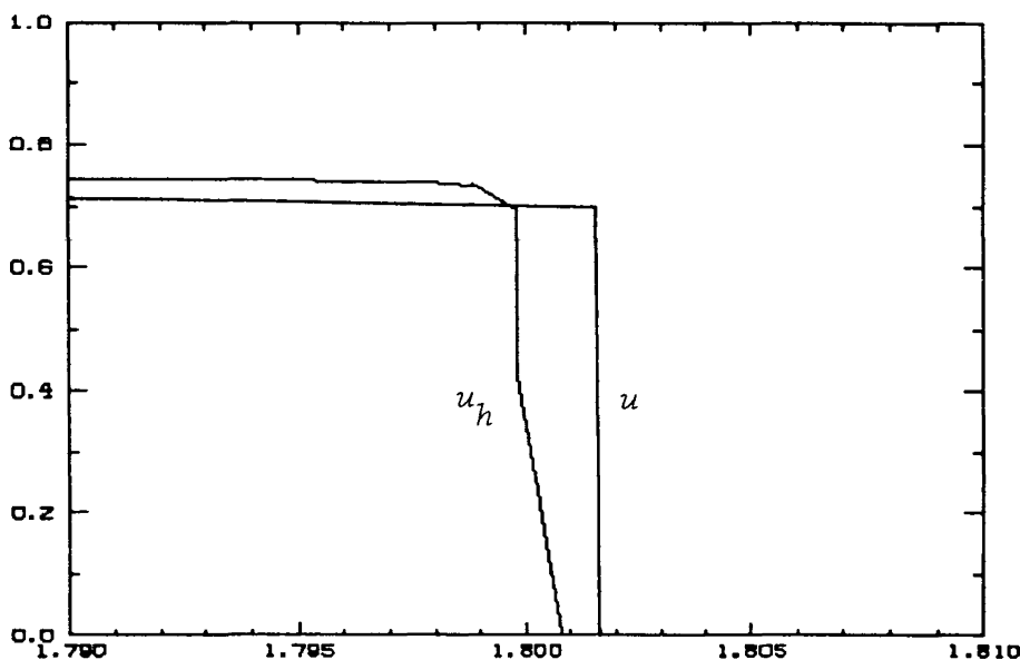
Figure 3.2a. — Detail of the convergence of the approximate solution determined by the \Lambda\Pi P^0 P^1 -scheme with \theta_i \equiv 1 , and cfl = 1/2 to a non entropy solution of the Buckley-Leverett problem 3.
