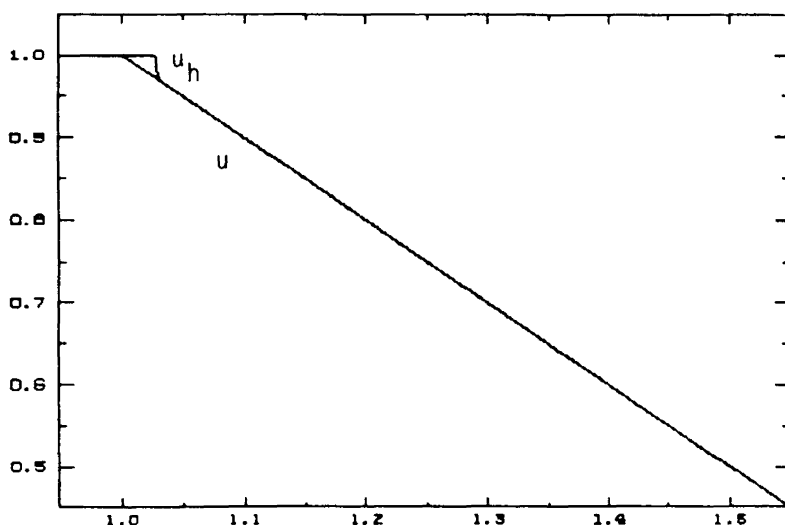
Figure 3.1b. — Convergence of the approximate solution determined by the \Lambda\Pi P^0 P^1 -scheme with \theta_i \equiv 1/2 , and cfl = 1/2 to the solution of the Burgers problem 2.
