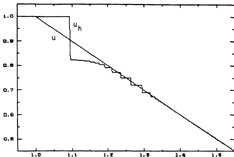
Figure 3.1a. — Convergence of the approximate solution determined by the \Lambda \Pi P^0 P^1 -scheme with \theta_i \equiv 1 , and cfl = 1/2 to a nonentropy weak solution of the Burgers problem 2.
