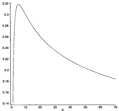
FIGURE 5. The ratio of the average Horton-Strahler number and the average stack-number.
