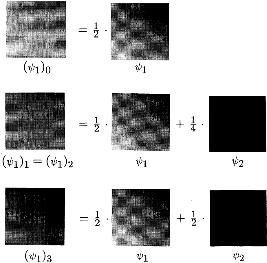
Figure 4. - Linear expressions defined by the outgoing transitions from state 1 in Figure 3.
