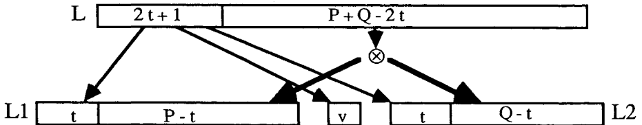
Schema of median-of- 2t + 1 partition
