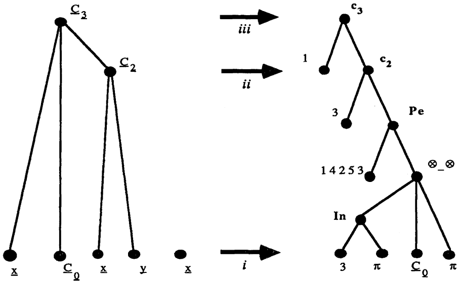
Figure 1. - Transformation of tuples of Herbrand terms into constant expressions.
