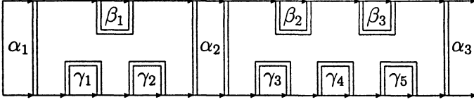
Figure 2: A composable arrangement in D[X] .
