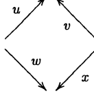
Figure 5: A false 1-globular cycle in the old globular homology
