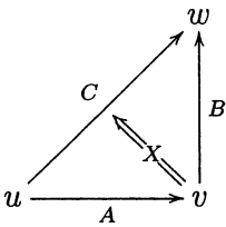
(a) A 2-globular simplex \tilde{X}
