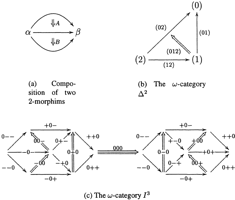
Figure 2: Some \omega -categories (a k -fold arrow symbolizes a k -morphism)
