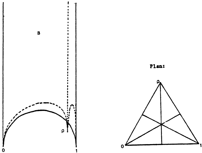
Figure 2.3.3. ( \alpha = \rho = \frac{1}{2}(1 + \sqrt{-3}) )
