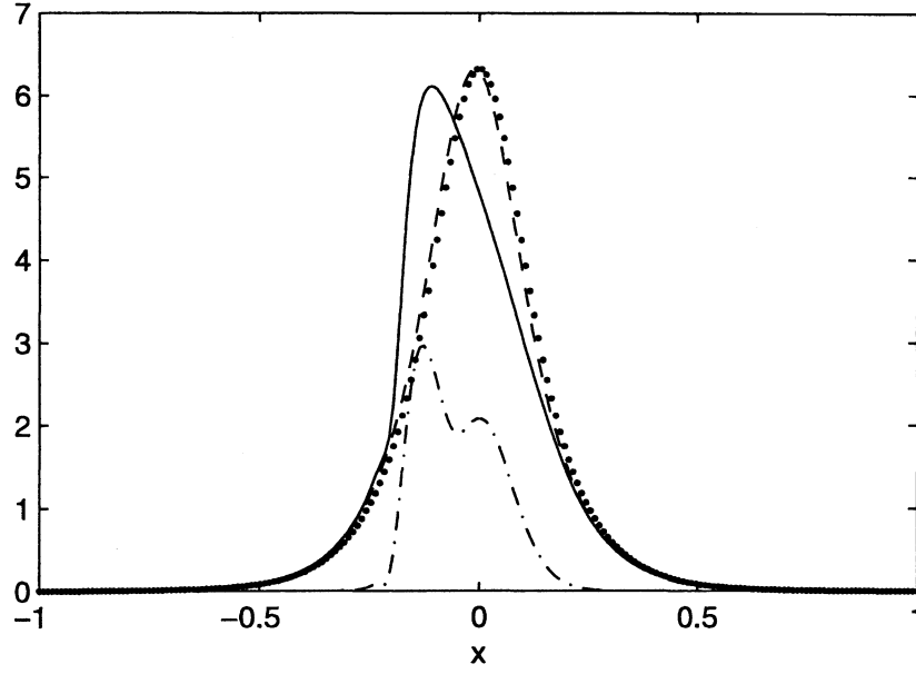
Fig. 1: |q_o| (dotted ..), |q(t_{max})| (continuous line -), |q_A(t_{max})| (dashed -) and |q(t_{max}) - q_A(t_{max})| (dashed-dotted .-) for: \epsilon = 0.1 , t_{max} = 0.01 , \Delta x = 0.01 , \Delta t = 1.10^{-5} , [a; b] = [-1; 1] , \Delta_\epsilon = 0.46 .
