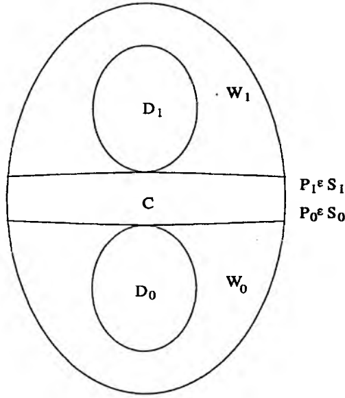
FIG. 5: Partition de \mathbb{P}(\mathbb{C}_p) .
