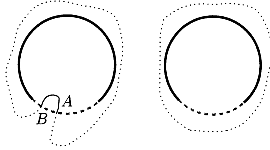
FIG. 1.5: Description (approximative) de \Sigma_i .
