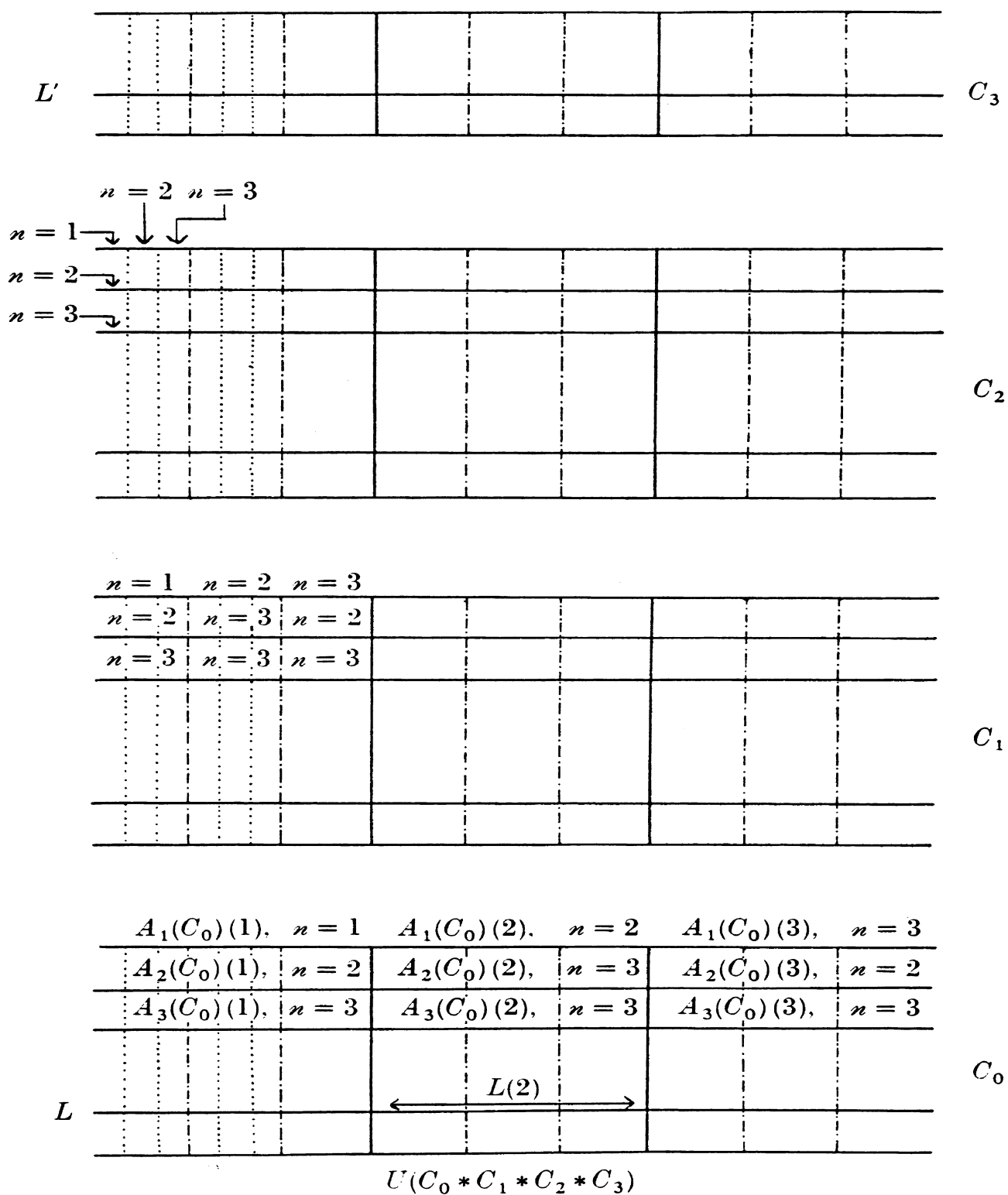
FIG. 2. Forming independent \alpha -blocks in C = C_0 * C_1 * C_2 * C_3 .
