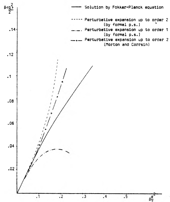
FIG. 2. Second steady-state moment of the solution of the equation \ddot{q} + \dot{q} + q + \beta q^3 = \dot{b}(t) , \langle b^2(t) \rangle = \sigma^2 |t| .
