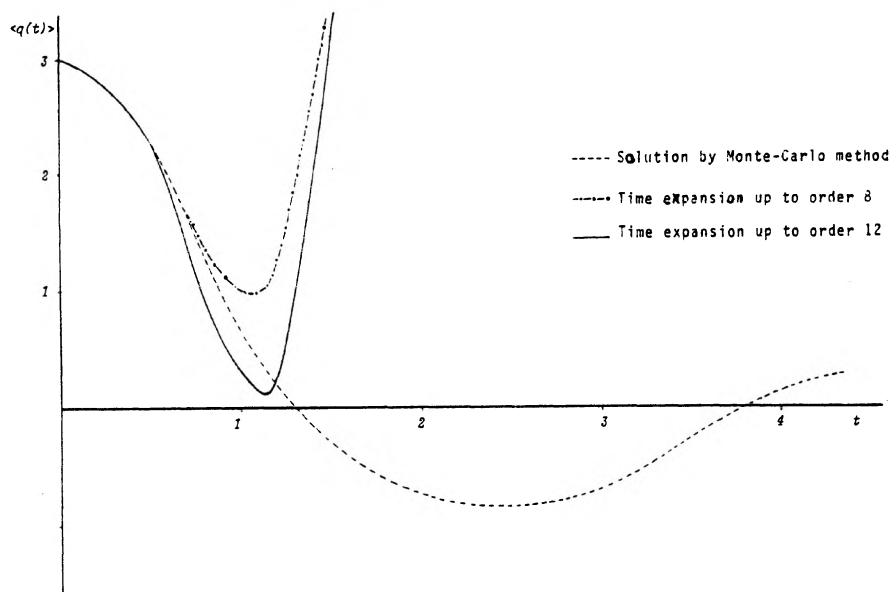
FIG. 1. First moment of the solution of the equation \ddot{q} + \dot{q} + q + 0.2q^3 = \dot{b}(t) with \sigma^2 = 5 , q(0) = 3 , \dot{q}(0) = 0 .
