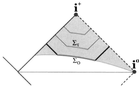
FIGURE 7B. Decay in Kerr can be measured with respect to a foliation \Sigma_\tau obtained from \Sigma_0 , by using the \mathbb{T} -flow. Note that \Sigma_0 consists of two null portions and a space-like one in the middle.
