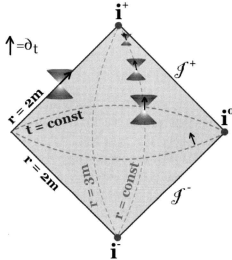
FIGURE 3B. The right disconnected exterior region of Schwarzschild. Note that \mathbb{T} = \partial_t becomes null along the horizon r = 2m and vanishes on the bifurcate sphere where the two branches of the horizon meet.
