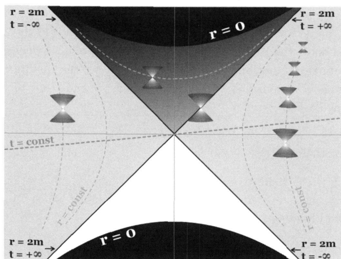
FIGURE 2. Kruskal's maximally extended Schwarzschild space-time. Note the two disconnected external regions, r > 2m , the black and white holes and the curvature singularity at r = 0 . Note the behavior of light cones at the event horizon, r = 2m .
