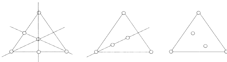
FIGURE 6. The configuration in the left naturally induces \mathcal{W}_{SK} while the one in the middle induces a 1-parameter family of exceptional webs.
