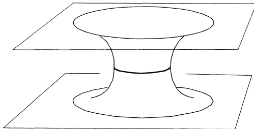
FIGURE 3. Two flat tori joined by a negatively curved tube.
