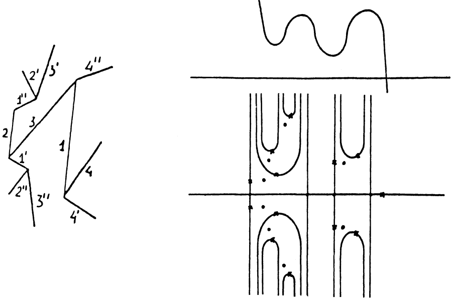
Figure 5 : A generic polynomial of degree 13, its monodromy tree , and its graph \Theta = P^{-1}(\mathbb{P}_R^1) .
