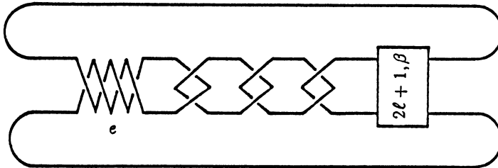
Montesinos link \mathbf{m}(0; \epsilon_0; 1/2, 1/2, 1/2, \beta/2\ell + 1) , e = \epsilon_0 + 3/2 + \beta/2\ell + 1 \in \mathbb{Z}
